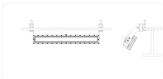
Clamp mount
