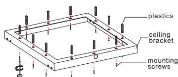
Schematic diagram for ceiling installation
