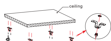
Schematic diagram for vertical installation
